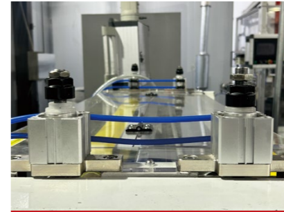
气动锁辊 Pneumatic lock shaft
