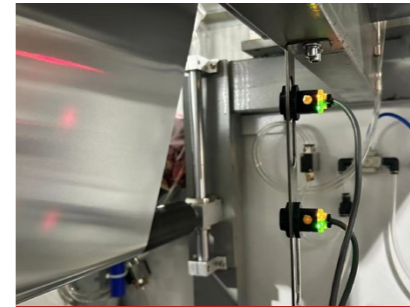
缺料自动报警 Lack of material detection
